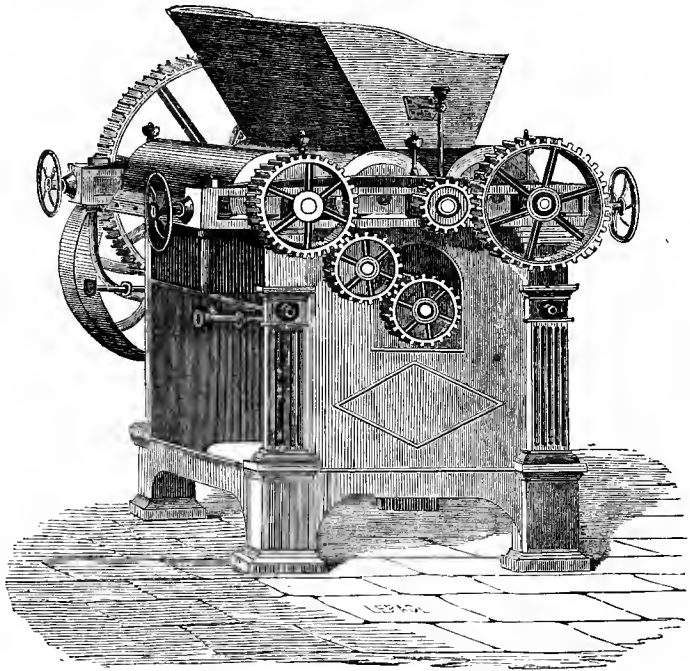
ROLLING-MACHINE. NO. 1.
